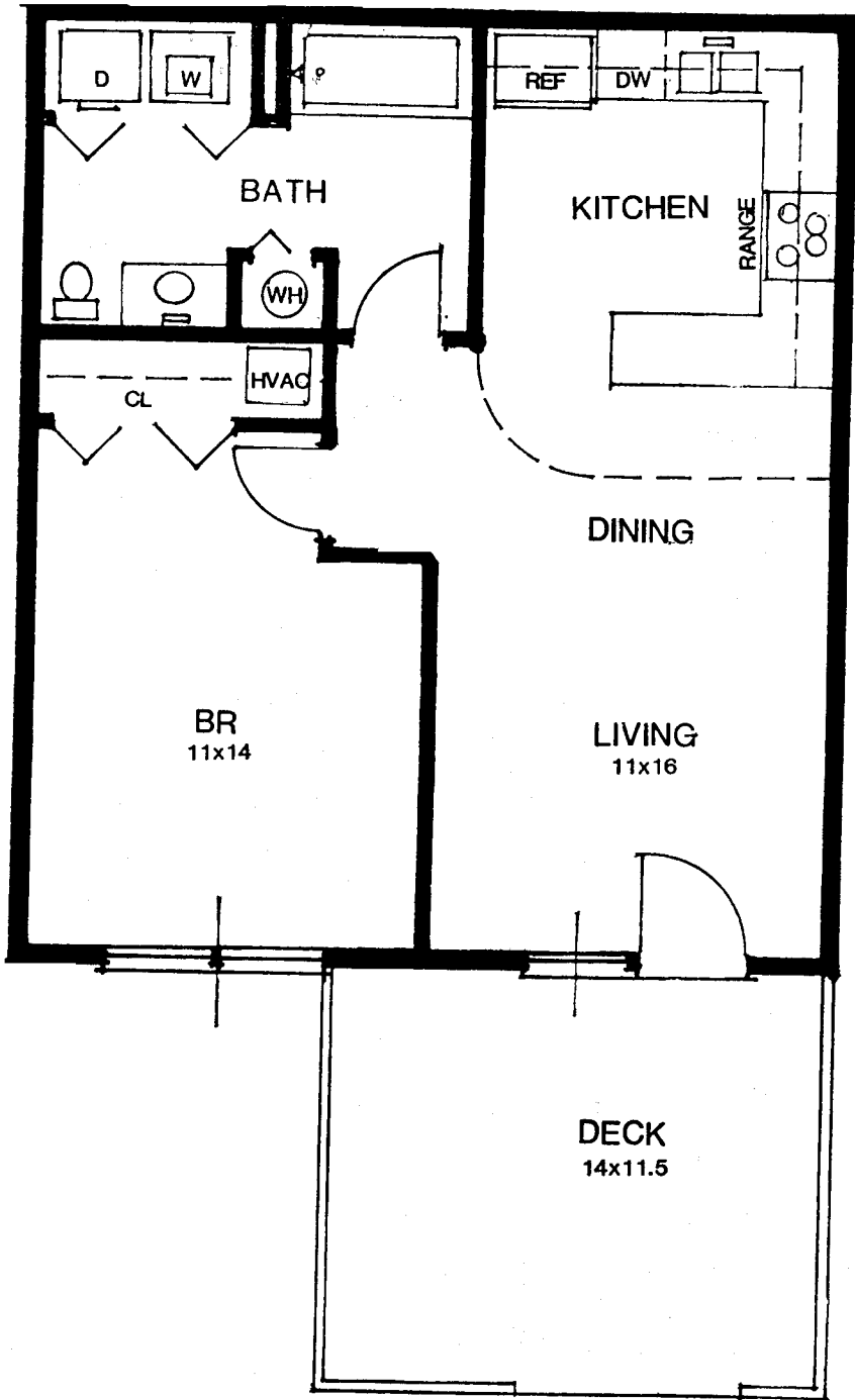
FLOOR PLAN
